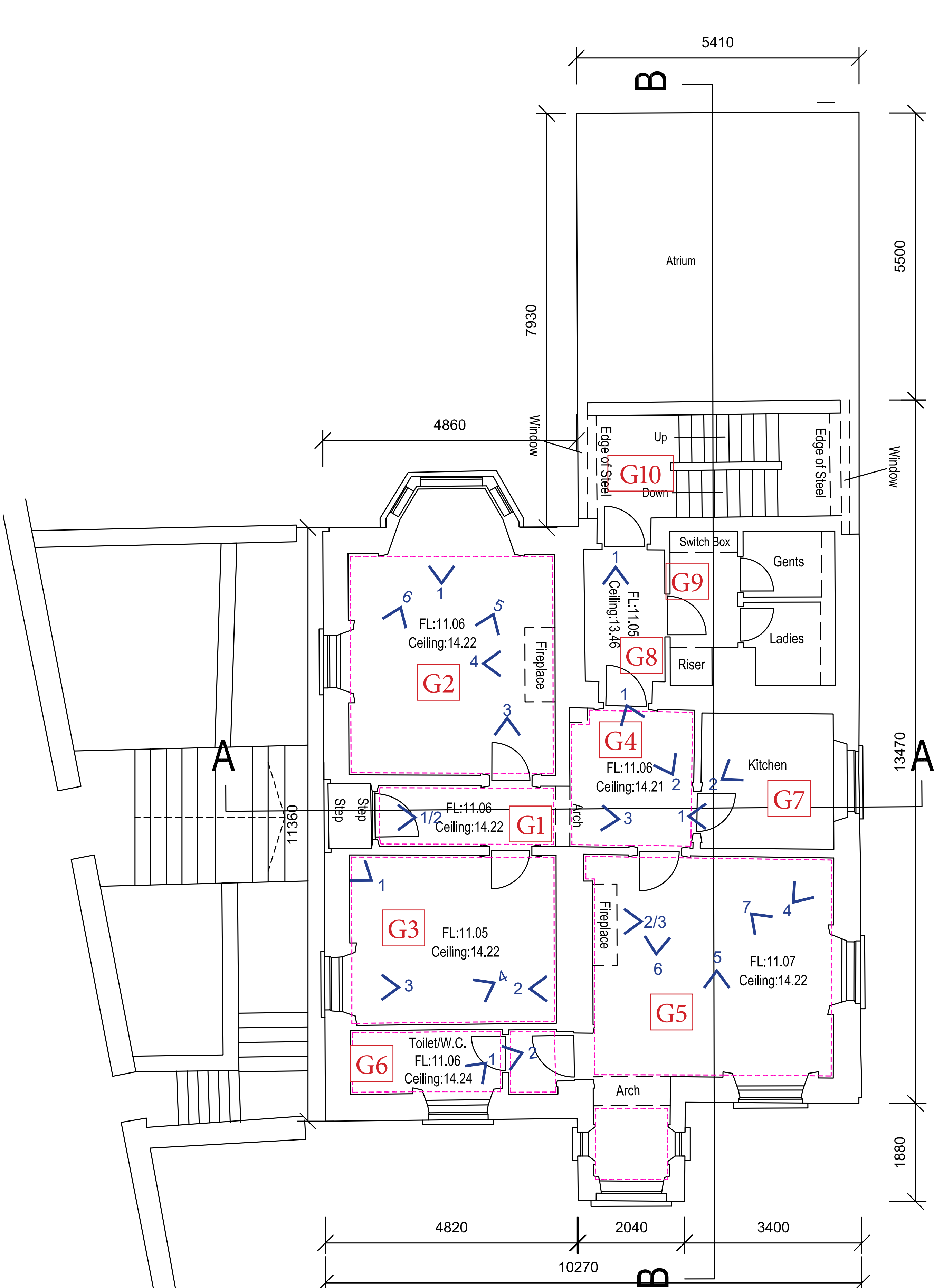
Existing Dun Leary House Level 02 (Ground Floor) 1:50
